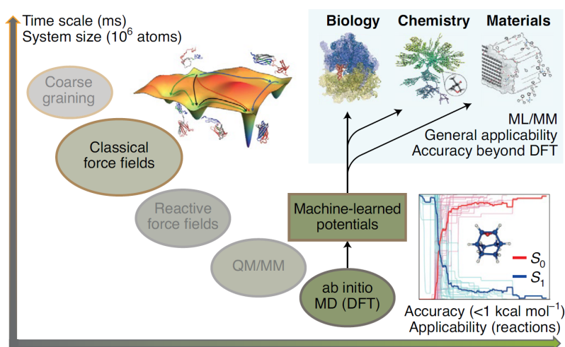
Figure 3: ML potentials as a potential solution to the trade-off between cost and accuracy of conventional atomistic simulations. Figure from Nature Mater. 20 (2021).
