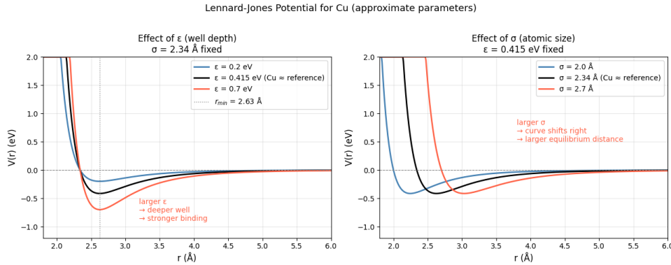
Figure 4: LJ potential curves as \epsilon and \sigma are varied.
