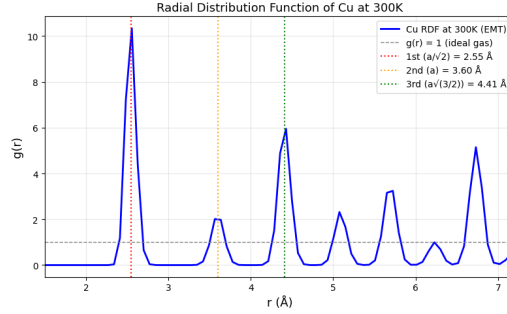
Figure 6: RDF of Cu FCC at 300 K (EMT). The first peak at \approx 2.55 \text{ \AA} corresponds to 12 nearest neighbours; thermal broadening produces Gaussian peaks.
